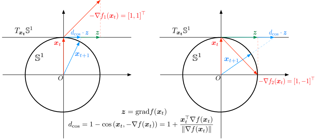
Figure 1: Example of modified Riemannian gradient descent on \mathbb{S}^1 . Without modification, two Euclidean descent directions -\nabla f_1(x_t) and -\nabla f_2(x_t) give the same Riemannian gradient z . We propose to multiply z with the cosine distance between x_t and -\nabla f(x_t) as the modified Riemannian gradient so that angular distances are taken into account during the parameter update.
